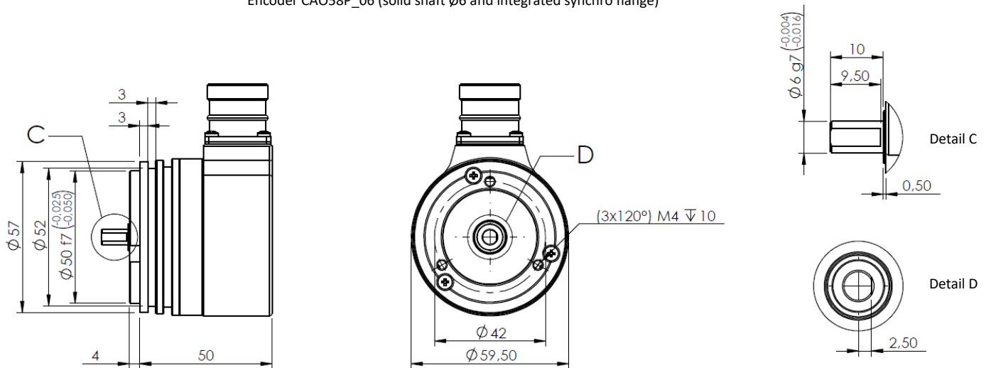
Encoder CA058P_06 (solid shaft Ø6 and integrated synchro flange)
