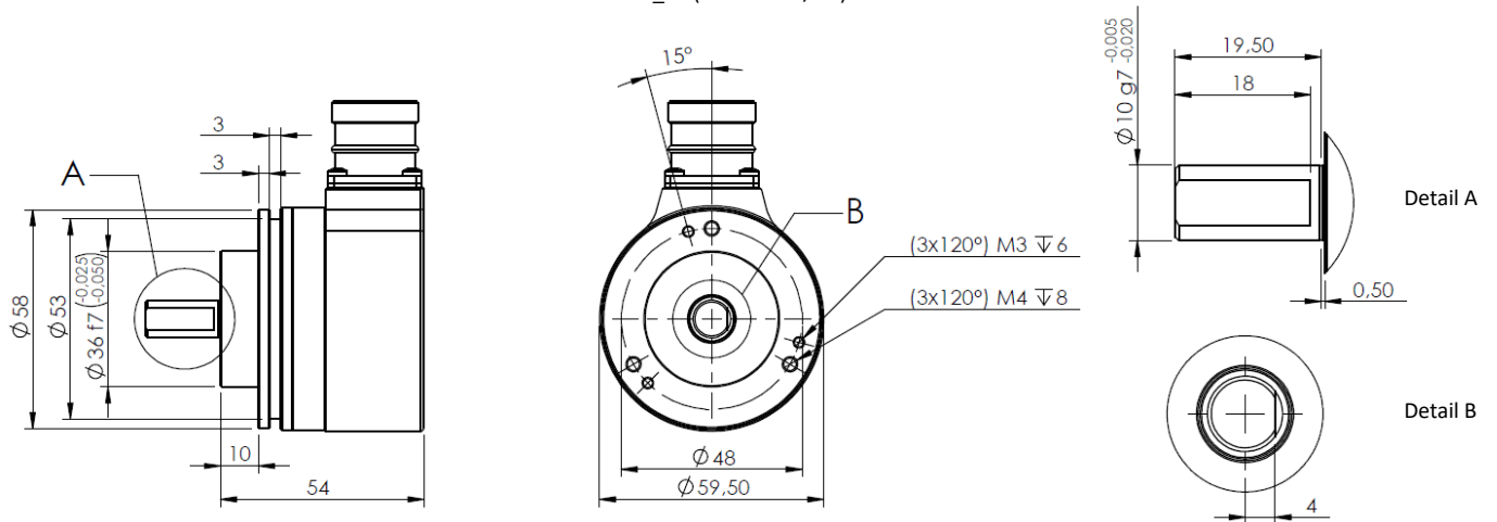
Encoder CA058P_10 (solid shaft Ø10)
